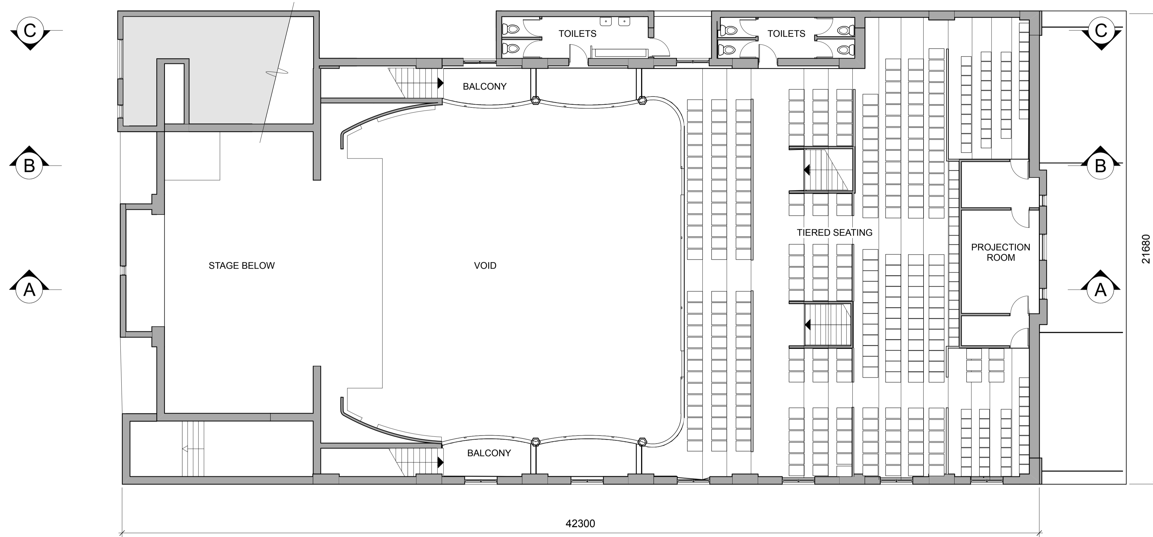
1 UPPER LEVEL PLAN - EXISTING
