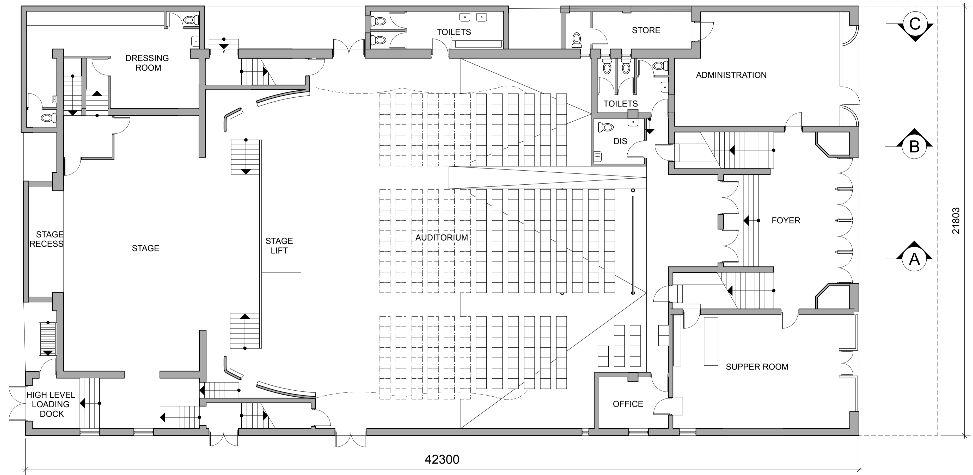
2 STAGE / DRESSING ROOM / LOWER LEVEL PLAN - EXISTING
